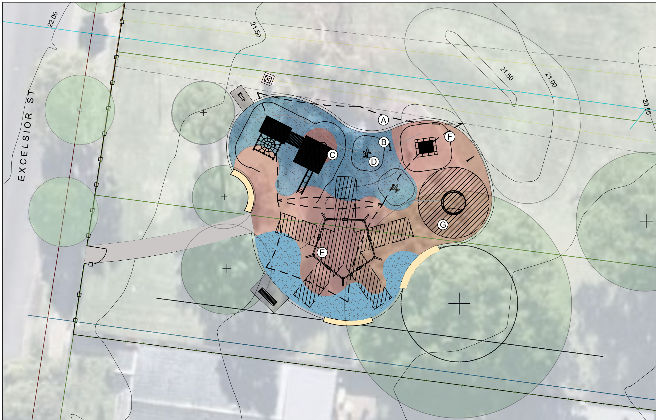
1 Equipment Plan Scale 1: 200
